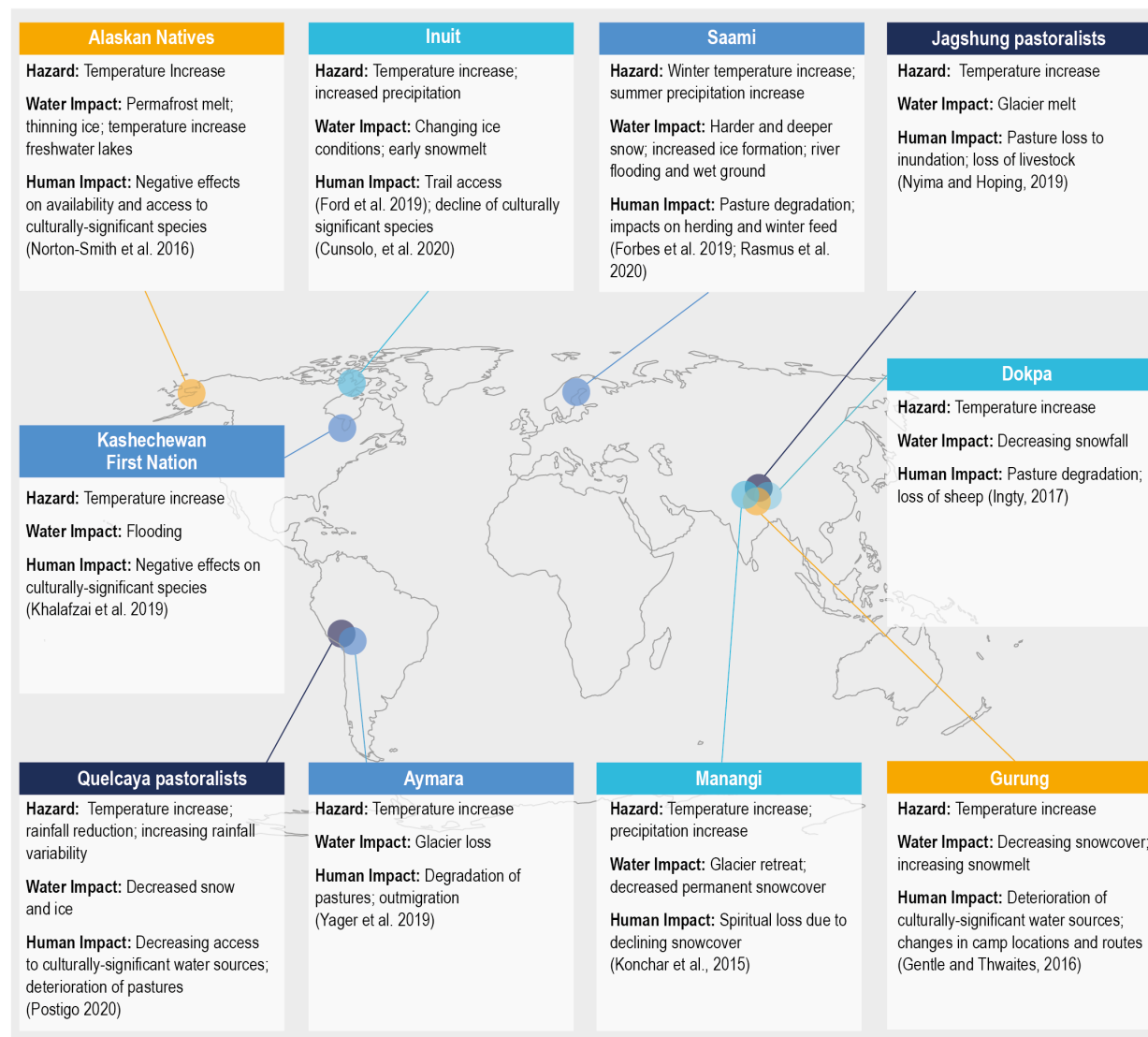
Map of selected observed impacts on cultural water uses of Indigenous Peoples of the cryosphere
