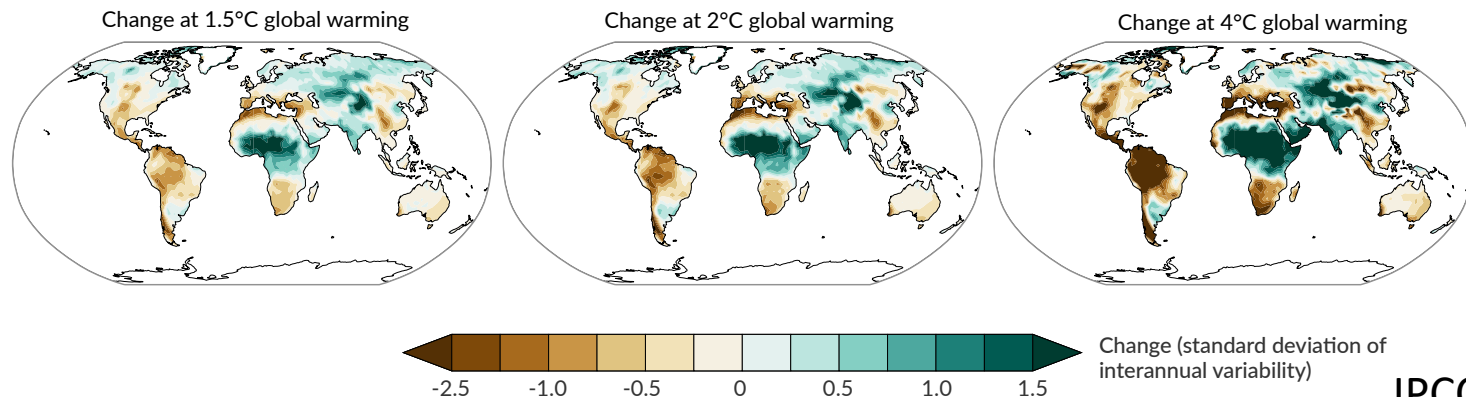
d) Annual mean soil moisture change (sd) (standard deviation of interannual variability) relative to 1850-1900 at three global warming levels
