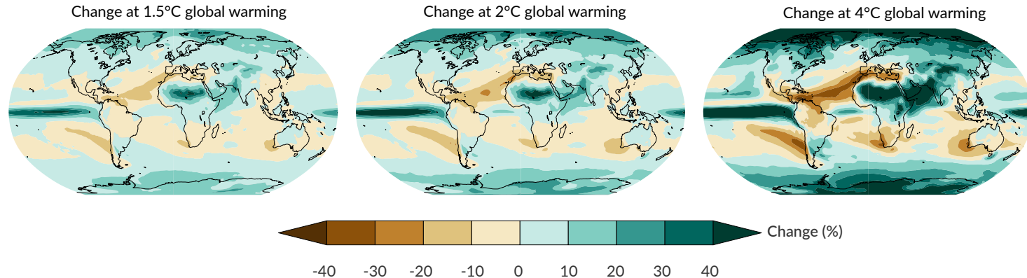
c) Annual mean precipitation change (%) relative to 1850-1900 at three global warming levels
